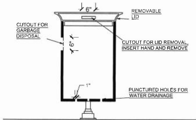
SIDE SECTION
